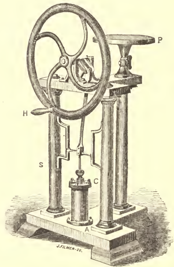
FIG. 4.—Large Improved Air Pump of Ritchie.
